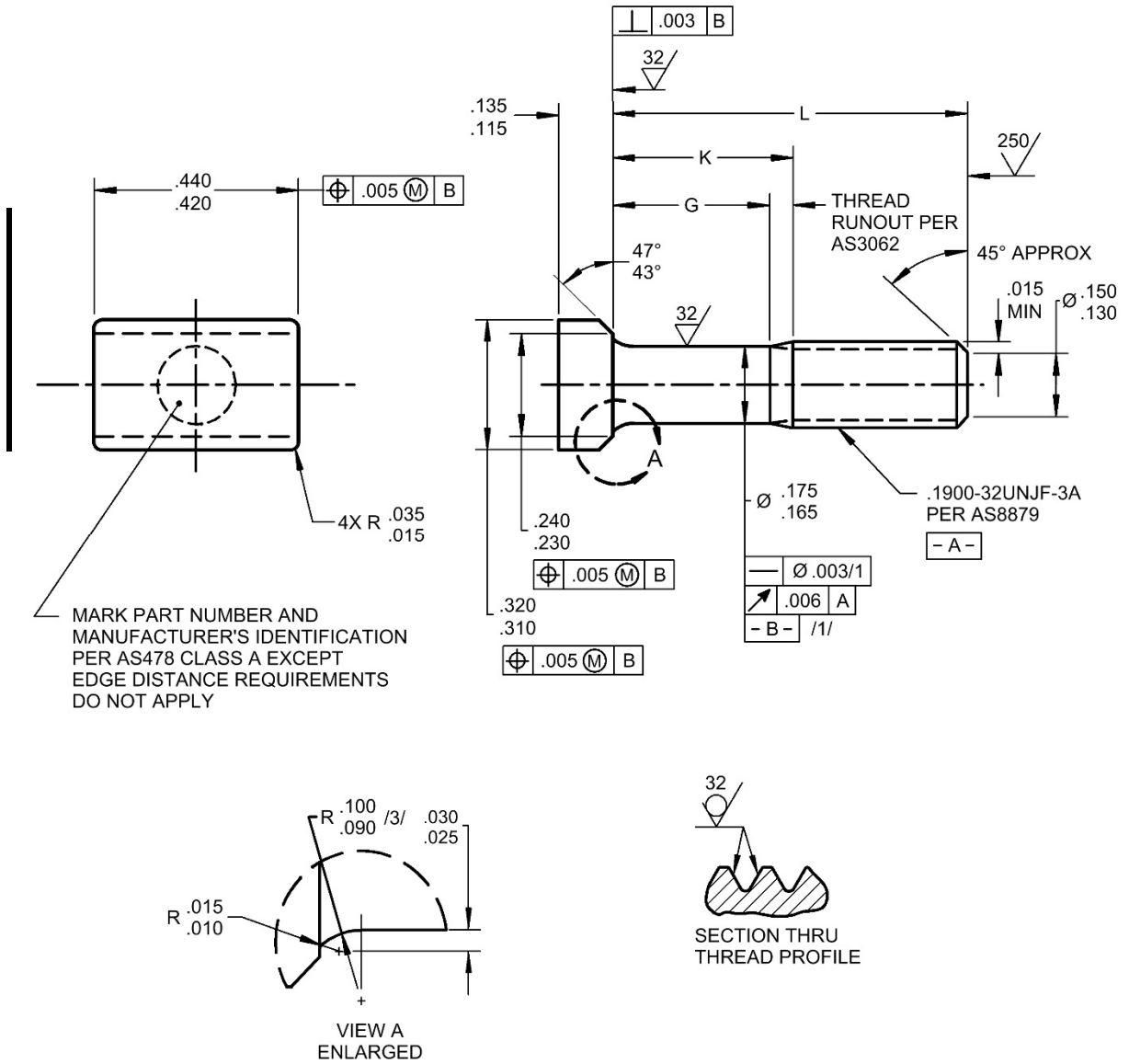
FIGURE 1 - BOLT
